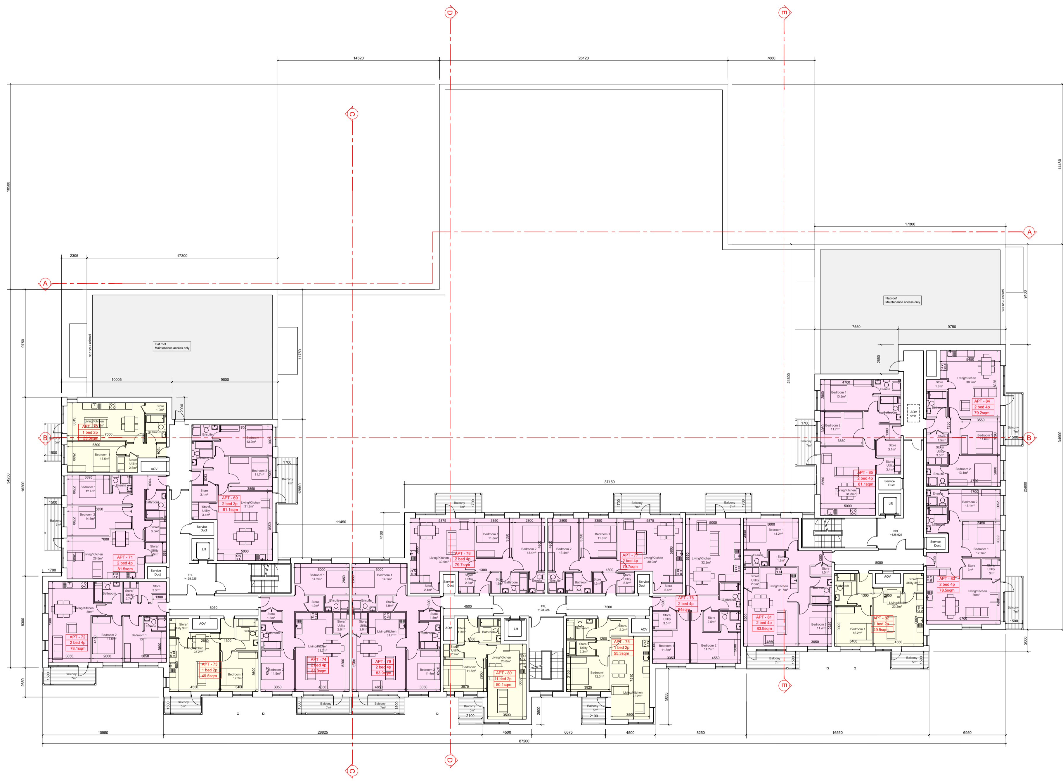
FOURTH FLOOR PLAN - 17 UNITS 5 - 1 BED APARTMENTS 12 - 2 BED APARTMENTS
