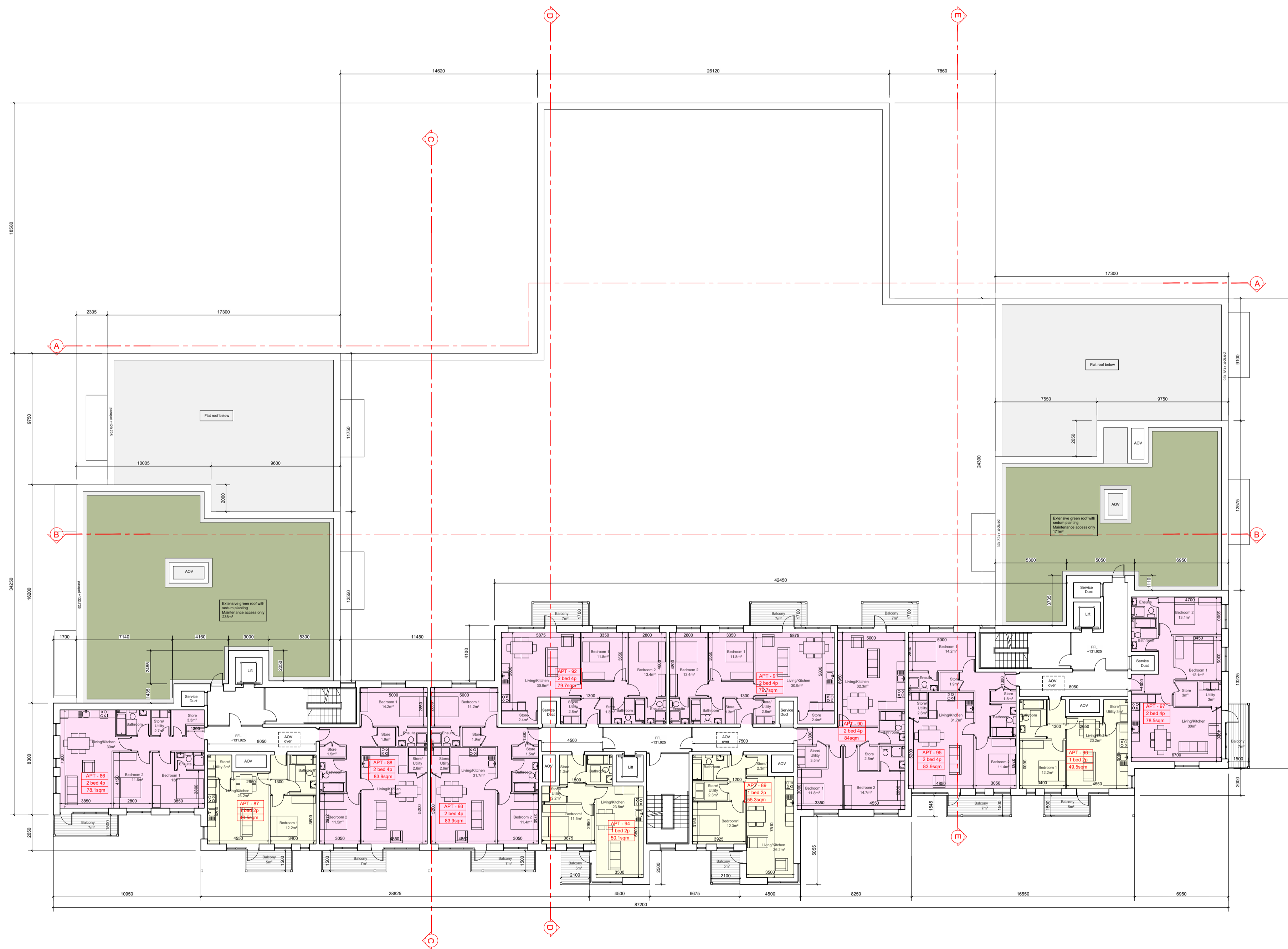
FIFTH FLOOR PLAN - 12 UNITS 4 - 1 BED APARTMENTS 8 - 2 BED APARTMENTS
