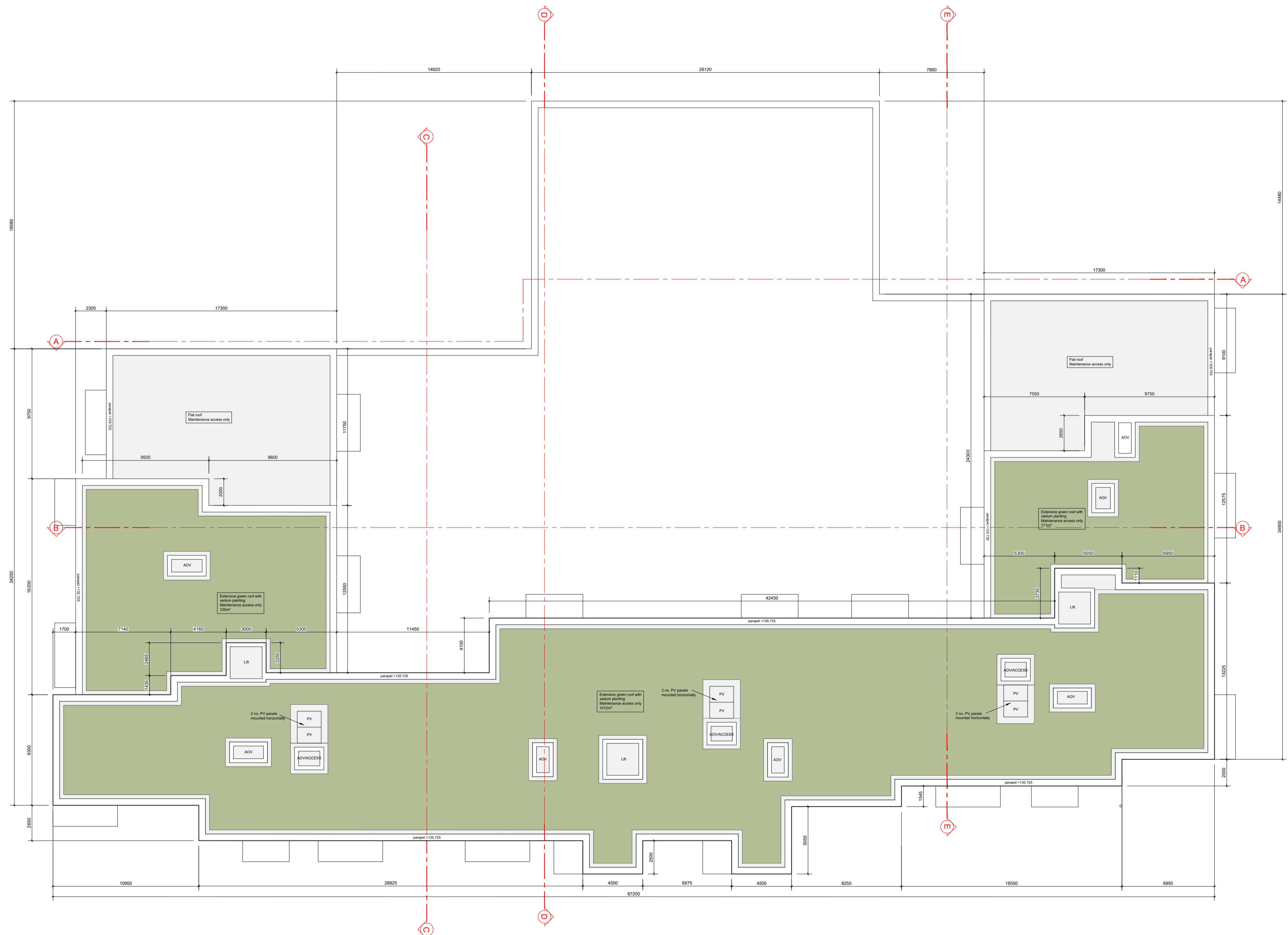
ROOF PLAN
